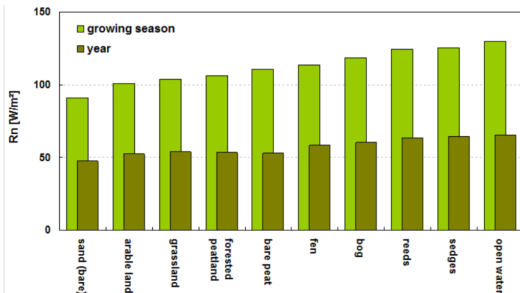
Figure 13: Net radiation for various types of land use in an example for the Marnitz climate station. Higher values correspond to lower warming of the lower atmosphere. Figure: K. Brust.
